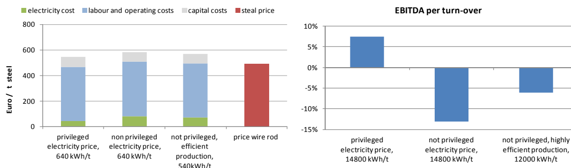
Figure 1: Left: product price and costs of EAF; Right: return (EBITDA) on turn-over of an aluminium producer Source: Data based on environmental and annual reports of companies in the steel and aluminium industry (2013/14). Notice: not all operating costs, e.g. for equipment and additional material, are included here.
